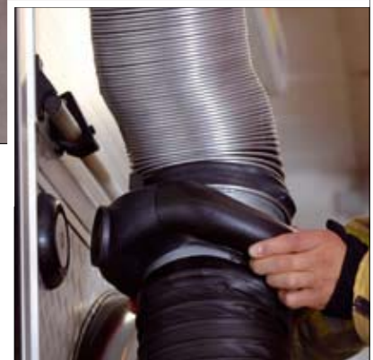
When activated, the electromagnet on the hose attaches to an anchor plate on the vehicle.
